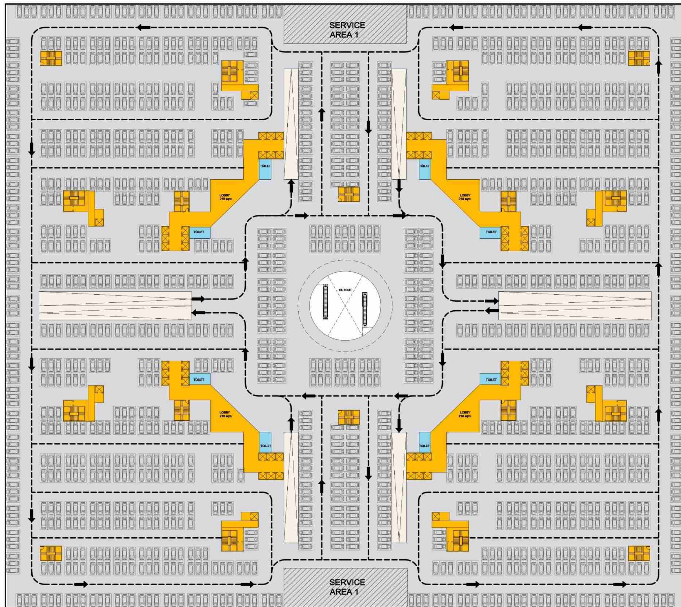
FIRST BASEMENT car 1400 nos FIRST BASEMENT PLAN
